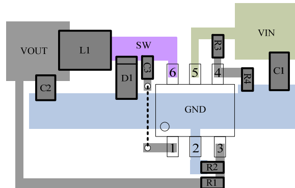
Figure 17. TRI1461 Recommended Layout Diagram
